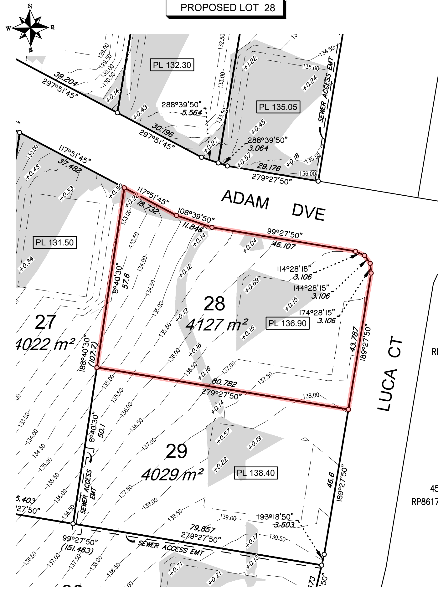
SCALE 1: 750 (A3) 15019-DP-28
