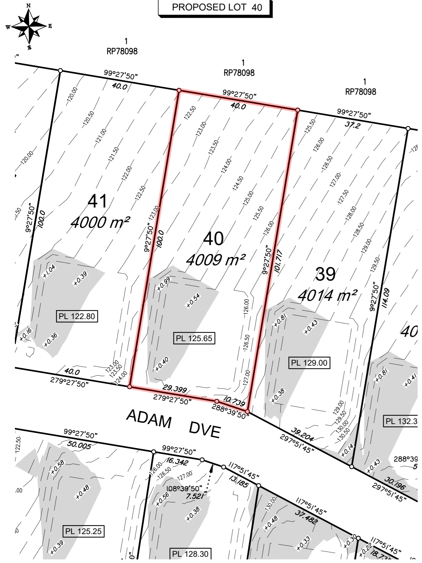
SCALE 1: 750 (A3) 15019-DP-40
