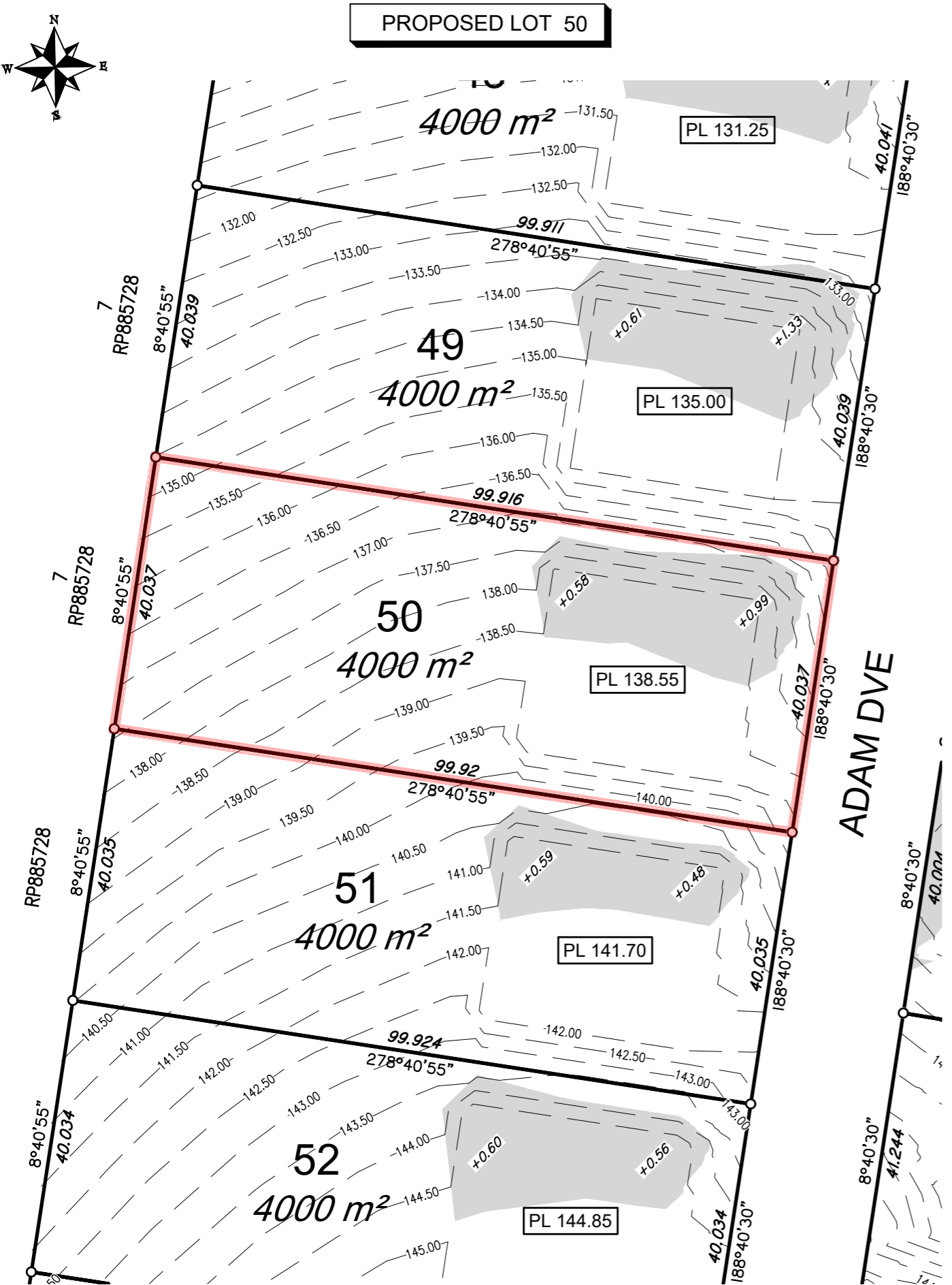
SCALE 1: 750 (A3) 15019-DP-50
